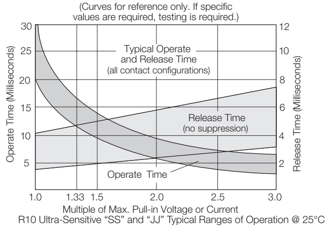
Operative Range R10 Relays (DC Only) Typical Ranges of Operations @ 25°C
